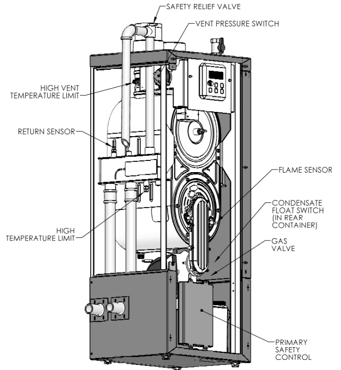
Figure 2: Control & Safety Device Locations – PF-210/399
