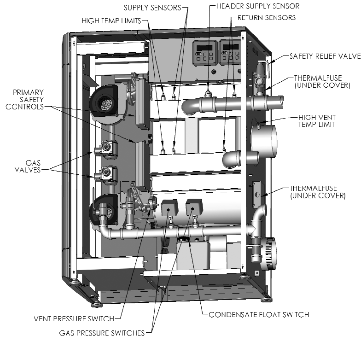
Figure 3: Control & Safety Device Locations – PF-850/1000
